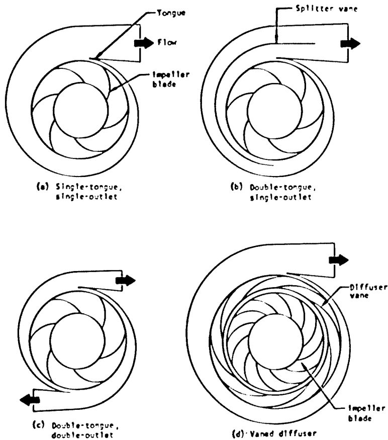
Figure 28. — Volute configurations.
