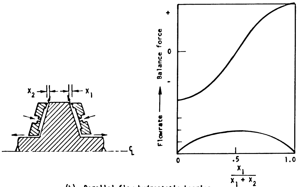
(b) Parallel-flow hydrostatic bearing
